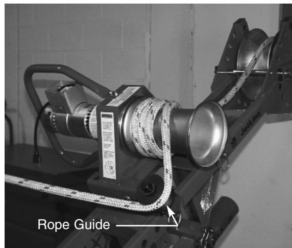
Rope Guide on CP800 Brutus Power Head
